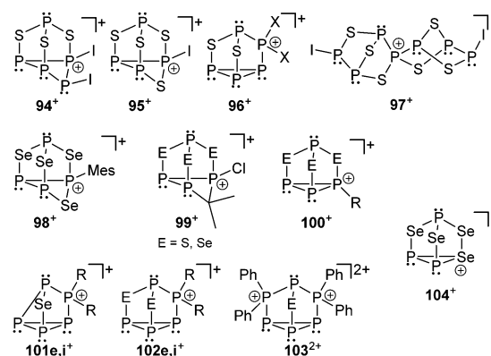
Fig. 17 Selected cationic polyphosphorus–chalcogen cages 94 + –103 2+ ( \text{E} = \text{S}, \text{Se} ) comprising bonding motif J ; cation 104 + has been included since it represents the first binary \text{SeP} -cation and is related to the other cations.
