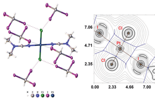
Fig. 1 Left: View of fragment 1a · (\text{CHI}_3)_6 from \mathbf{1a} \cdot \frac{1}{2}\text{CHI}_3 \cdot 1\frac{1}{2}\text{CHI}_3 . Thermal ellipsoids are shown with 50% probability and short contacts are indicated by dotted lines. Coordinates of this fragment were applied in further DFT calculations. Right: Contour line diagram of the Laplacian distribution \nabla^2\rho(r) (cross-section along the plane \text{Pt–Cl–I} ) was received as a result of the topological analysis of the electron density distribution in the model structure. Bond paths are shown as brown lines, selected zero-flux surfaces – as blue lines, bond critical points (3, –1) are shown in blue, nuclear critical points (3, –3) – in pale brown, length unit – Å.
