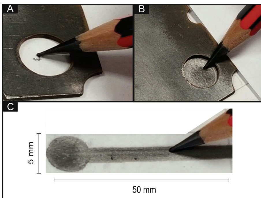
Fig. 1 Optical image of the bespoke metallic stencil used throughout this work (A) to fabricate the PDEs. Shown in (B) is the PDE after one draw, and the completed PDE with a connecting strip is shown in (C). Sellotape® was applied to each individual electrode to cover the conductive carbon connections and define the 4 mm working area.
