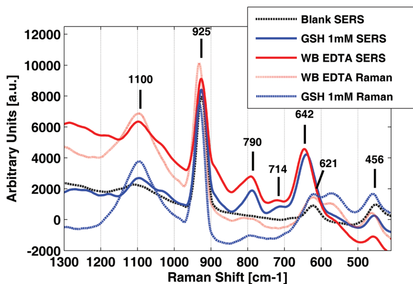
Fig. 1 SERS and Raman spectra of a glutathione (GSH) standard solution and a K 2 -EDTA whole blood (WB) sample in comparison with a H 2 O blank.
