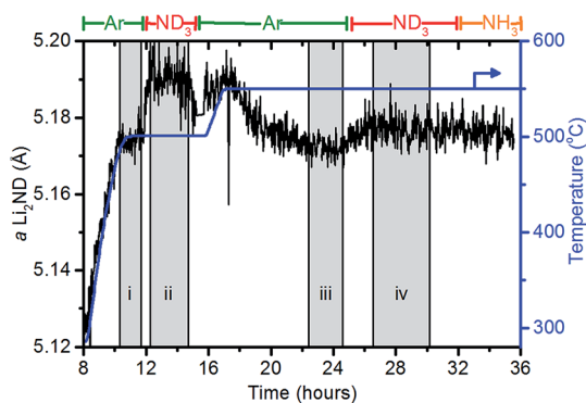
Fig. 6 Variation of the a lattice parameter of Li 2 ND (black) over the course of the experiment. The temperature of the sample (blue) is shown for comparison. Shaded areas represent periods of NPD data which were summed and analysed for the sample stoichiometry.
