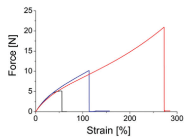
Fig. 7 Lap shear tests on cured rubbers: (a) comparison between DA- (blue) and DTDB- (red) cured rubbers, adhesion for 30 min at 180 °C, (b) DTDB-cured rubber adhered at 180 °C for varying times (pink: 5 min, green: 10 min, blue: 20 min and red: 30 min), (c) DTDB-cured rubber adhered for 30 min at different temperatures (black: 100 °C, blue: 150 °C and red: 180 °C).
