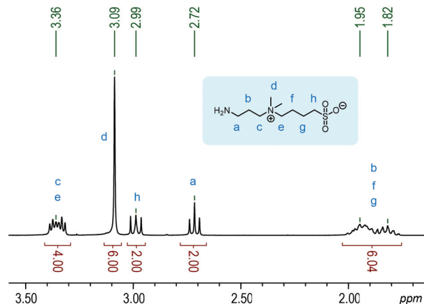
Fig. 6 ^1\text{H} NMR spectrum of sulfobutylbetaine amine recorded in \text{D}_2\text{O} .
