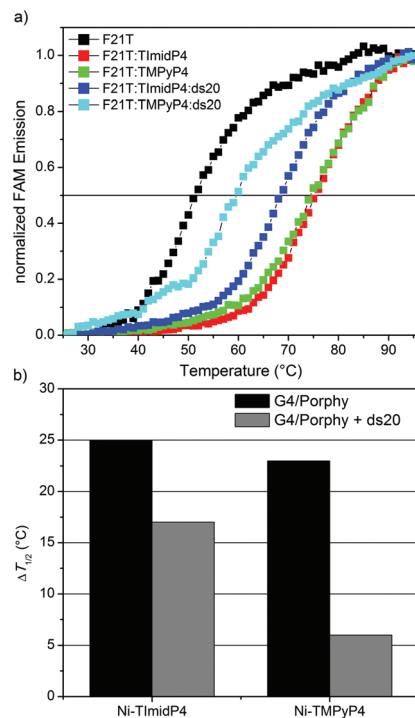
Fig. 3 (a) Melting curves of 200 nM pure F21T and in the presence of a 1 μM Ni II -TlmidP4 ligand or a 1 μM Ni II -TMPyP4 ligand without or with the presence of 15 equiv. of competitor double-stranded DNA (ds20). The curves shown correspond to normalized FAM fluorescence. (b) Melting temperature differences ΔT 1/2 from FRET melting assays for each metalloporphyrin without and with the presence of the competitor ds20. All measurements were performed in a 10 mM lithium cacodylate buffer (pH = 7.2) with 10 mM KCl and 90 mM LiCl.
