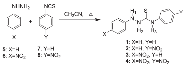
Scheme 1 Synthesis of the thiosemicarbazide anion sensors 1–4 in dry \text{CH}_3\text{CN} on refluxing for 2 hours.
