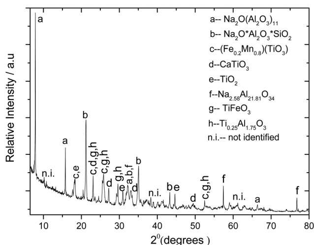
Fig. 10 X-ray powder diffraction of alkali roasted red mud and bauxite samples at 775 °C in air before water leaching. The diffraction data compare well with the ICDD references: 01-072-0587 ( \text{Na}_2\text{O}(\text{Al}_2\text{O}_3)_{11} ), 04-011-8808 ( \text{TiFeO}_3 ), 04-002-8136 ( \text{Ti}_{0.25}\text{Al}_{1.75}\text{O}_3 ), 04-017-0197 ( (\text{Fe}_{0.2}\text{Mn}_{0.8}\text{TiO}_3) ), 00-030-1148 ( \text{Na}_2\text{O}.\text{Al}_2\text{O}_3.\text{SiO}_2 ), 04-004-3579 ( \text{TiO}_2 ), 04-011-8342 ( \text{CaTiO}_3 ), and 00-037-1460 \text{Na}_{2.58}\text{Al}_{21.81}\text{O}_{34} .
