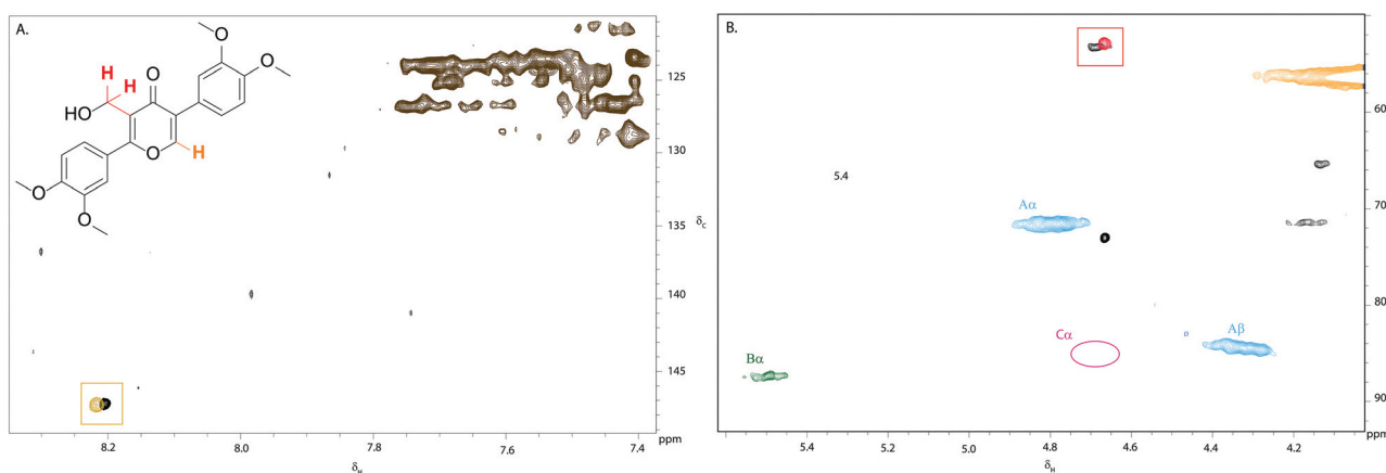
Fig. 5 Overlay of partial 2D HSQC NMR spectra of (i) Kraft lignin after treatment with 0.75 weight equivalents of DDQ and (ii) of an authentic sample of pyran-4-one 5 : (A) aromatic region ( \delta_c/\delta_H 120–150/7.4–8.4) and (B) aliphatic region ( \delta_c/\delta_H 50–90/4.0–5.6). The close proximity of the aromatic and methylene cross peaks in 5 with new cross peaks present in the DDQ-treated lignin spectrum are shown in orange and red boxes respectively. Contours are colour coded according to the linkage they are assigned to (see Fig. 2 legend).
