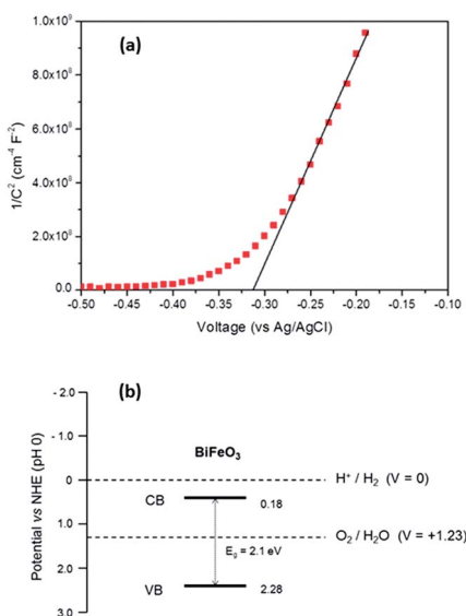
Fig. 3 (a) Mott–Schottky plot for \text{BiFeO}_3 electrode measured in the dark using 0.2 \text{ M Na}_2\text{SO}_4 at pH 6.5, (b) schematic illustration of the estimated location of the conduction and valence bands in \text{BiFeO}_3 with respect to the redox potentials of water splitting.
