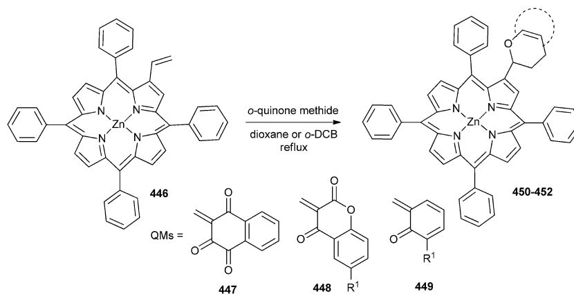
Scheme 98 Hetero-Diels-Alder reaction of o -QMs with \beta -vinyl- meso tetraphenylporphyrinatozinc(II).
