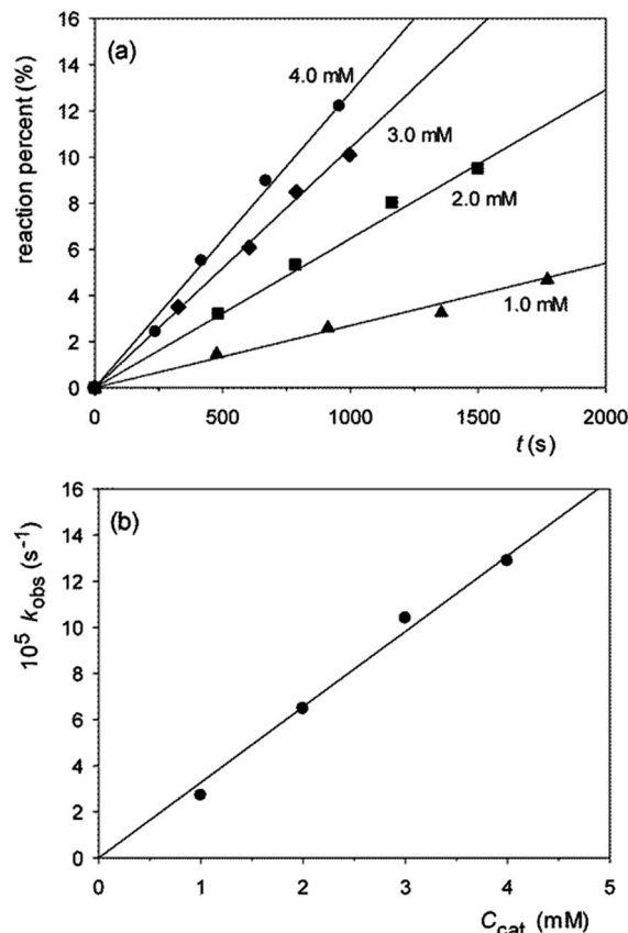
Fig. 2 Cleavage of 0.10 mM GpU catalyzed by 1.0–4.0 mM 1 (80% DMSO, pH 10.4, 10 mM Me 4 NClO 4 , 50.0 °C). (a) Reaction percent vs. time, for experiments carried out at the given catalyst concentration. (b) Plot of k_{\text{obs}} vs. total catalyst concentration C_{\text{cat}} .
