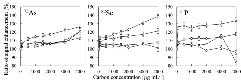
Fig. 8 Signal enhancement ratios of 75 As, 82 Se and 31 P as a function of carbon concentration for different pH values: (□) pH 2; (△) pH 4; (◇) pH 6; and (○) pH 8. Error bars indicate standard deviation ( n = 3 ). Oxalic acid was used for a carbon source and pH adjustment was conducted by adding \text{HNO}_3 or \text{NH}_4\text{OH} .
