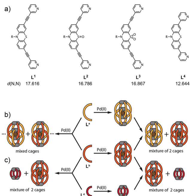
Fig. 1 (a) Chemical structures of the cage-forming ligands L^1 – L^4 . The given N,N -distances are based on double-cage X-ray structures for L^1 – L^3 and a semiempirical PM6 model for the monomeric cage based on ligand L^4 . (b) For binary systems containing two different long ligands L^a + L^b ( L^a, L^b = L^1 – L^3 ; L^a \neq L^b ) the outcome of the self-assembly gives mixed cages showing a statistical ligand distribution when the ligands are mixed prior to the addition of palladium. In contrast, combining two preassembled double-cages [Pd_4L^a_8] + [Pd_4L^b_8] leads to a mixture of coexisting homogeneous structures between which ligand exchange is tremendously slowed down. (c) For binary systems containing one long ligand ( L^b = L^1 – L^3 ) and the short ligand L^4 , the outcome of the self-assembly is independent of the order of mixing of the components. In both cases, this system shows narcissistic self-sorting behaviour to give [Pd_4L^b_8] + [Pd_2L^4_4] .
