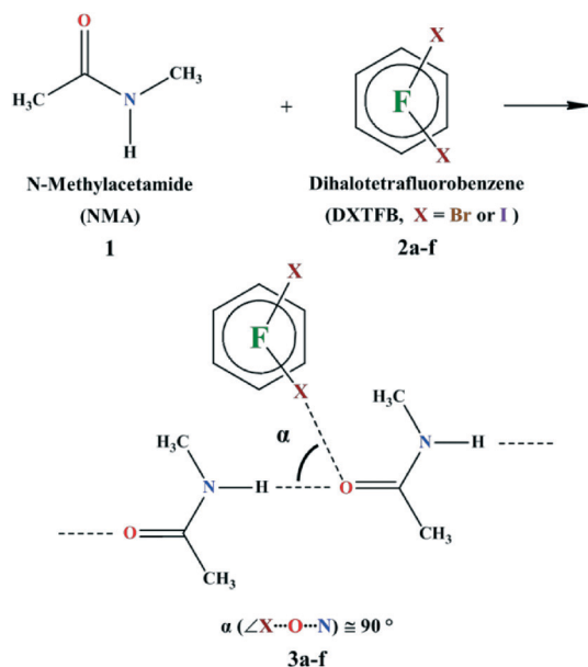
Scheme 1 Synthesis of N -methylacetamide (NMA, 1 ) co-crystals with various dihalotetrafluorobenzenes (DXTFB, 2a-f , X = Br or I). The orthogonal angle ( \alpha ) is defined as the angle between XB (C-X \cdots O, X = Br or I) and HB (N-H \cdots O), i.e., \angle X\cdots O\cdots N .
