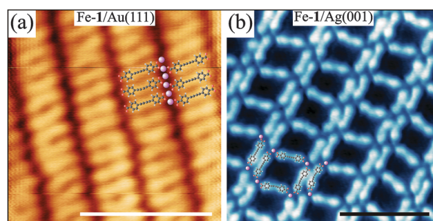
Fig. 2 (a) Fe-rich row phase on Au(111). Fe : 1 ratio 2 : 1. (b) Fe-deficient double-row structure on Ag(001). Fe : 1 ratio 2 : 3. Structures were obtained by simultaneous deposition of Fe and 1 at 450 K. Images acquired at 5 K. Scale bars are 5 nm.
