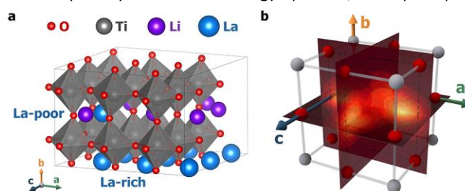
Fig. 1 (a) A 3-dimensional representation of the LLTO structure; (b) An illustration of a Ti 8 cage where the metadynamics simulations were carried out. Three collective variables were constructed to represent the a, b, and c coordinates of Li + within the cube; see the main text and ESI for details. Planar slices of the 3D free-energy profiles normal to the three axes were visualized in Fig. 2, with those at T = 100 K shown here as a visual reference.
