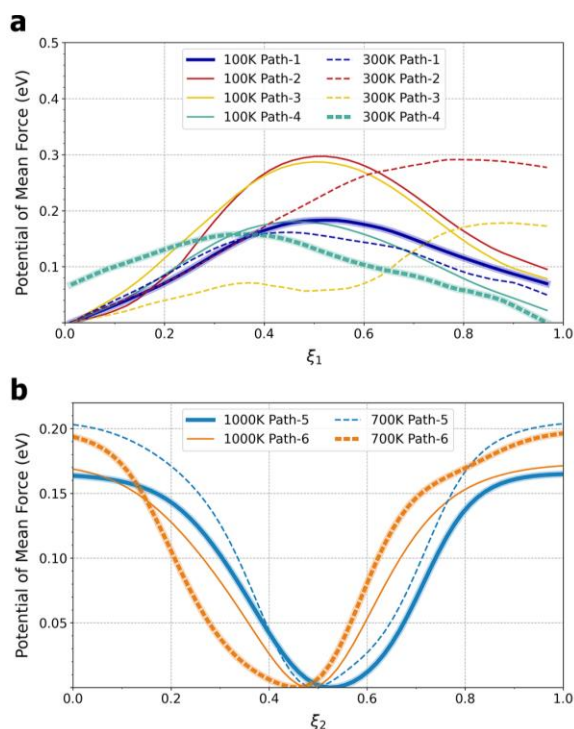
Fig. 3 Free-energy profiles along (a) pathways 1 – 4 at T = 100 and 300 K and (b) pathways 5 and 6 at T = 700 and 1000 K. The bold lines indicate the minimum-free-barrier pathways. See Fig. S1 for the definition of pathways. Note that \xi_1 , as defined by Eqn. (4) in the SI, does not start at 0 or end at 1.
