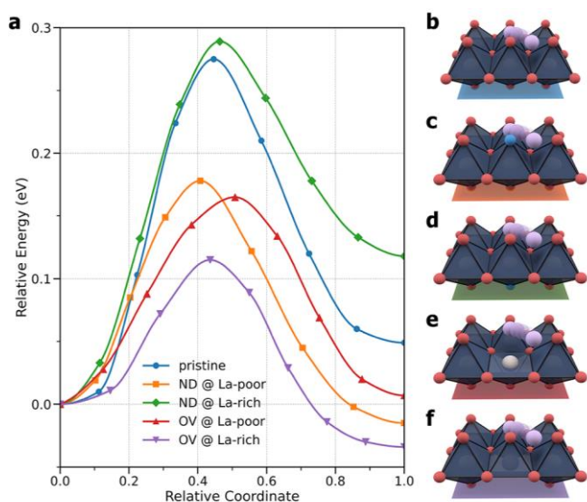
Fig. 4 (a) Potential energy profiles for minimum-energy \text{Li}^+ migration pathways in pristine LLTO, LLTO with a nitrogen dopant (ND) in La-poor and La-rich layers, and LLTO with an oxygen vacancy (OV) in the La-poor and La-rich layers; (b-f) Illustration of \text{Li}^+ hopping pathways examined for (b) pristine, (c) ND@La-poor, (d) ND@La-rich, (e) OV@La-poor, and (f) OV@La-rich structures.
