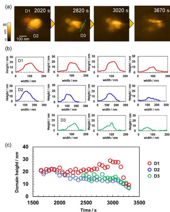
Fig. 6. HS-AFM analysis of the degradation behavior of the spherical degradation products at 30 °C in the presence of 62.5 mM NaO 4 : (a) height images, (b) cross-sectional profiles corresponding to each line in (a), and (c) changes in the domain size during degradation.
