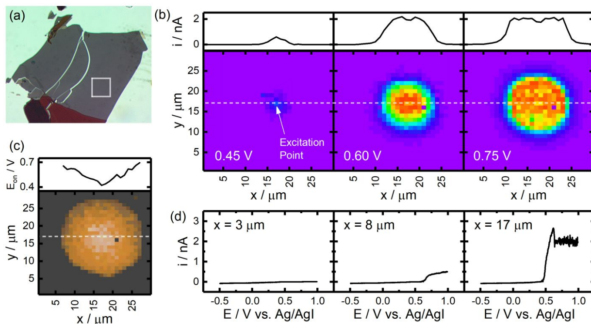
Figure 2. CG-TC SECCM imaging of transport with bulk n-WSe 2 . (a) Optical transmission image of an exfoliated n-WSe 2 flake with a thickness of 25 nm. The region within this flake interrogated via SECCM is indicated. (b) Photocurrent images at different potentials obtained in the vicinity of a focused 633 nm laser (1.12 μW). (c) Image of onset potentials ( E_{on} ), calculated as the potential necessary to reach a current of 100 pA. (d) Voltammograms obtained at different points along the dashed line in (b). The sweep rate was 0.20 V s -1 . All SECCM data was obtained using a ~600 nm diameter probe filled with 0.1 M NaI, 0.01 M I 2 .
