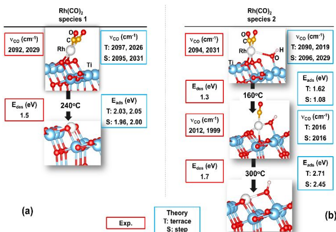
Fig. 3 Structure of \text{Rh}(\text{CO})_2 species identified by FTIR-TPD spectra and DFT calculations and evolution with temperature on (a) (Rh)ads and (b) (RhOH)ads species. Red boxes (left): experimental results; blue boxes (right): DFT results.
