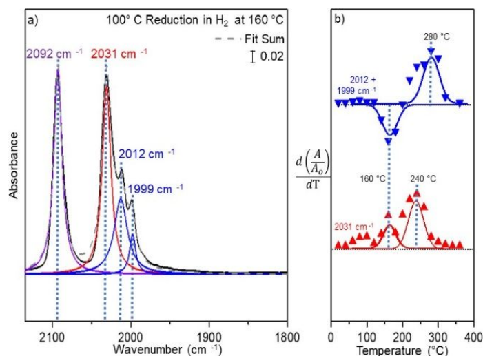
Fig 2. a) CO probe molecule FTIR spectra of sample reduced in \text{H}_2 at 100 °C taken during CO TPD at 160 °C. Peaks were deconvoluted from the original spectra in black, with the \text{Rh}(\text{CO})_2 symmetric stretch at 2092 \text{cm}^{-1} in purple, the \text{Rh}(\text{CO})_2 asymmetric stretch at 2031 \text{cm}^{-1} in red, and bands formed at 2012 and 1999 \text{cm}^{-1} in blue. b) Comparison of temperature dependent rate of change in normalized CO band intensity ( A/A_0 ) for the asymmetric stretch (2031 \text{cm}^{-1} , red) and newly formed features (2012 and 1999 \text{cm}^{-1} , blue). Maxima and minima in the rate of change, associated with the formation and loss of species, are highlighted at characteristic temperatures.
