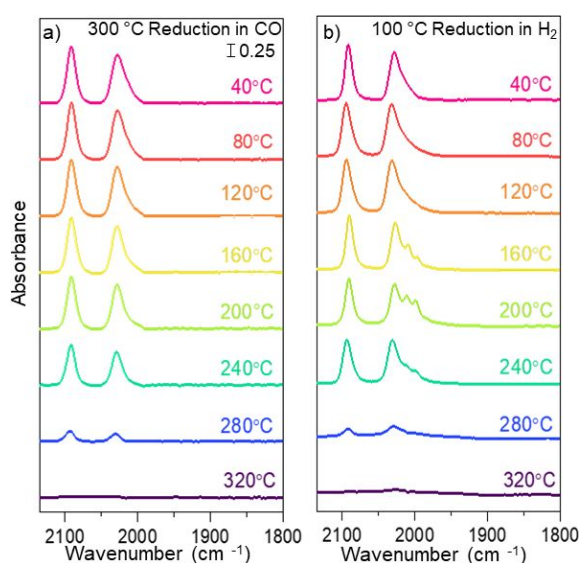
Fig. 1 FTIR spectra following CO saturation and during a TPD of CO from Rh(CO) 2 supported on anatase TiO 2 following varied pre-treatment conditions: a) reduction in CO at 300 °C and b) reduction in H 2 at 100 °C.
