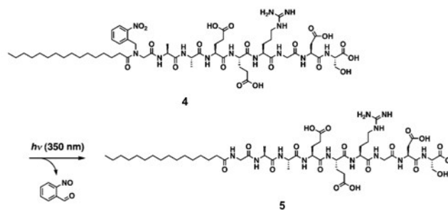
Figure 20 Irradiation of a peptide amphiphile results in cleavage of the 2-nitrobenzyl group and hence gelation. Reproduced from Ref. 137 . Copyright (2009) with permission from John Wiley and Sons.
