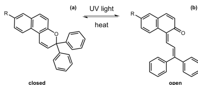
Figure 13 Molecular structure change of 2H-chromene from the (a) closed to the (b) open form.
