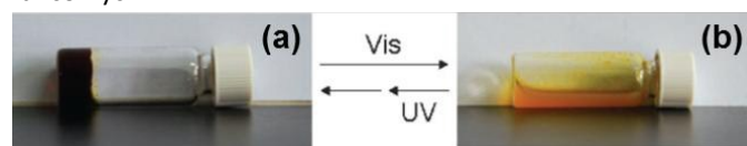
Figure 12 Photographs of (a) open spiroyrans gel and (b) closed spiroyrans solution open irradiated with different light sources. Adapted from Ref. 96 with permission of the Royal Society of Chemistry.
