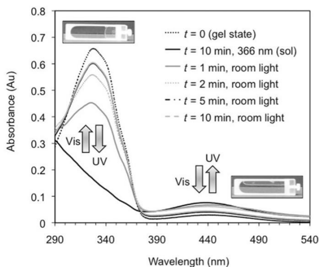
Figure 4 Reversible changes in the UV/Vis spectra for an organogel in toluene showing the reversible trans -to- cis isomerisation of the azobenzene moiety. On irradiation with UV light, the trans isomer changes to the cis isomer, leading to a gel-to-sol transition. Reproduced from Ref. 54 with permission from the Royal Society of Chemistry.
