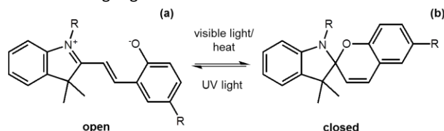
Figure 11 Molecular structure of a spiroyrans molecule (a) in the open form and (b) the closed form.
