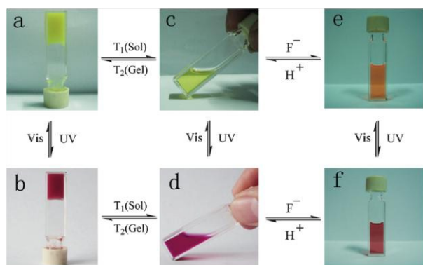
Figure 10 Colour change and state change upon different stimuli for a naphthalimide and cholesterol appended dithienylethene gelator. Reproduced from Fig. 97 with permission of the Royal Society of Chemistry.
