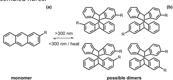
Figure 16 Dimerisation using >300 nm of anthracene from the (a) monomer to (b) the dimer.
