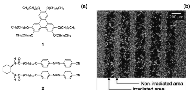
Figure 5 (a) Molecular structures of 1 and 2 (b) Optical polarized light microscope image of a patterned sample of 1,2 at 65 °C prepared by cooling under UV light using a photomask. Adapted from Ref. 74 with permission from the Royal Society of Chemistry.
