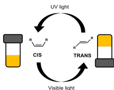
Figure 3 Switching between two isomers of the same molecule, the gel forming trans -isomer and the non-gelling cis -isomer, using light.
