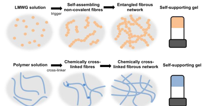
Figure 1 Gelation using (top) low molecular weight gelators, where the cross-links are generally formed by entanglement and (bottom) polymers, where the cross-links can be permanent chemical bonds or entanglements.
