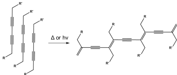
Figure 18 UV-polymerisation of a diacetylene-containing LMWG leads to a polymeric network being formed.
