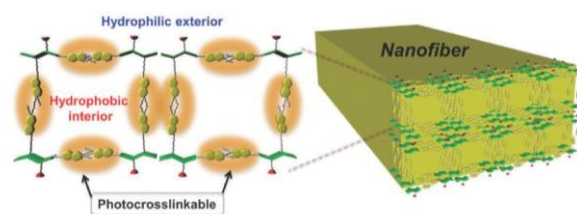
Figure 15 Diagram showing the possible cross-linking within a fibre due to coumarin dimerisation of the dipeptide functionalised hydrogelator. Reproduced from Ref. 106 with permission from the Centre de la Recherche Scientifique (CNRS) and the Royal Society of Chemistry.
