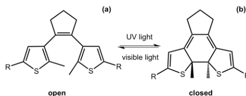
Figure 9 Molecular structure of dithienylethene in (a) the open form and (b) the closed form.
