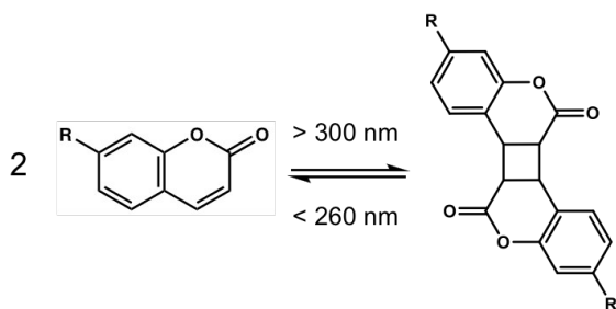
Figure 14 The reversible photodimerisation of a coumarin from (a) the monomer to (b) the dimer.
