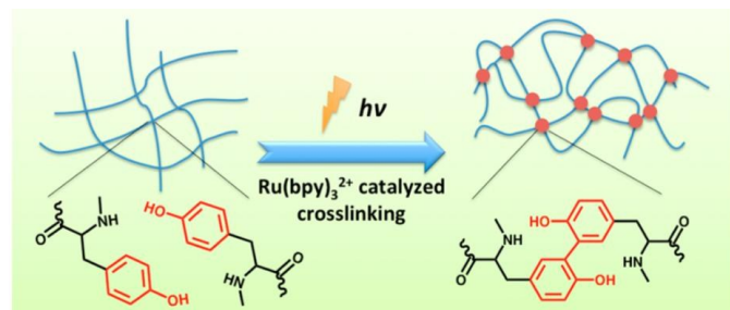
Figure 19 Irradiation of a tyrosine-containing LMWG in the presence of a ruthenium catalyst leads to cross-linking and a dramatic increase in gel strength. Reproduced from Ref. 135 with permission of the Royal Society of Chemistry.
