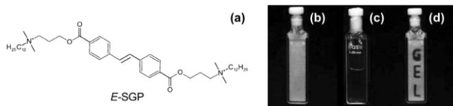
Figure 8 Molecular structure of alkene-based photoresponsive LMWG. On exposure to UV light, a trans -to- cis isomerisation occurs, leading to a gel-to-sol transition. Reproduced from Ref. 35 with permission of the Royal Society of Chemistry.
