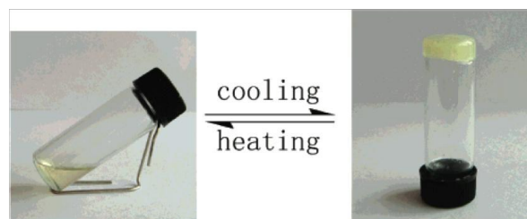
Figure 17 Gelation of urea functionalised anthracene molecule in dichloroethane using a heat-cool method. Adapted from Ref. 119 with permission of the Royal Society of Chemistry.
