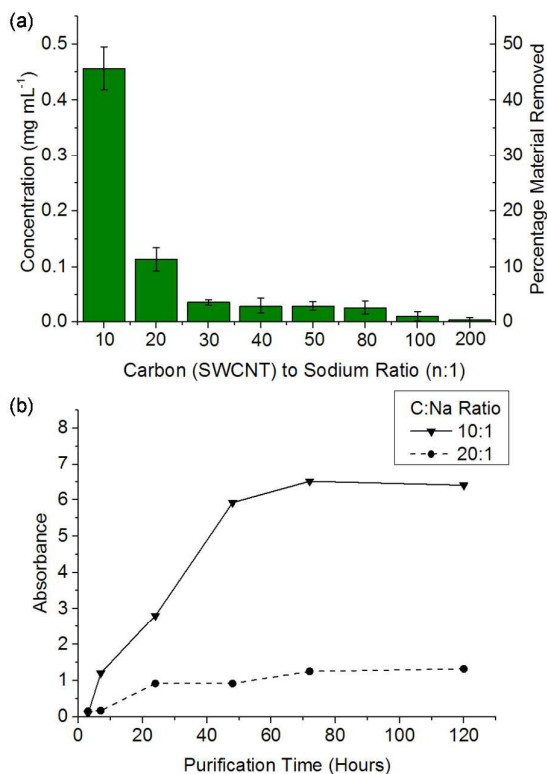
Figure 6. (a) Concentration of material dissolved versus C/Na after 48 h soaking of 1 mg mL -1 SWCNT in DMAc. (b) Absorbance (660 nm) of NaNp/DMAc and SWCNTs at a given SWCNT to sodium ratio versus time.
