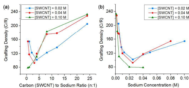
Figure 5. Grafting density of reduced SWCNTs added to 1-bromododecane versus (a) C:Na ratio, (b) sodium concentration, illustrating a shifting ideal stoichiometry but a stable sodium concentration
