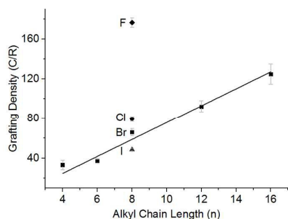
Figure 4. Grafting density of alkyl halides as a function of alkyl chain length ( C_nH_{2n+1}Br ) and halide; C_nH_{17}X where X = F (◆) Cl, (●), Br (■) or I (▲) for 20:1 charged SWCNTs. Line fitted to alkyl bromide series.
