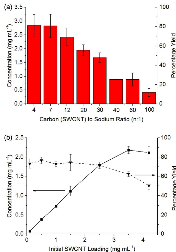
Figure 3. (a) Influence of C:Na ratio on the concentration of nanotubide solution starting with 3.5 mg mL -1 loading of SWCNT. (b) The yield and concentration of nanotubide solutions against initial SWCNT loadings with 20:1 C/Na. Error bars represent standard deviations of 3 repeats.
