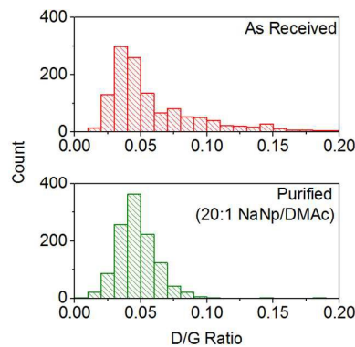
Figure 7. Distribution of D/G Raman ratios of Elicarb SWCNTs before and after Na-np purification (20:1 purification, 633 nm excitation). D/G of as received SWCNTs = 0.06 \pm 0.037 , D/G of as purified SWCNTs = 0.047 \pm 0.015 .
