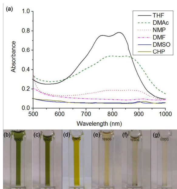
Figure 2. (a) UV-Vis spectra of equimolar sodium and naphthalene (of ~1 mg(Na) mL^{-1} ) added to a selection of solvents. (b-g) Cuvettes containing the Na + Np solutions of (b) THF (c) DMAc (d) DMF (e) NMP (f) DMSO (g) CHP
