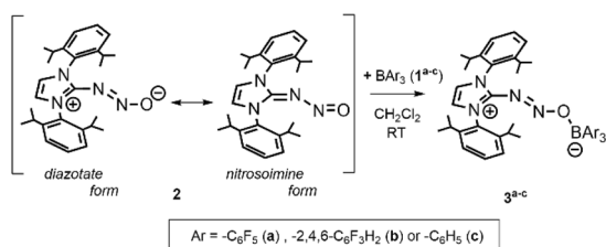
Scheme 2 Synthesis of the IDipp· N_2O · Bar_3 compounds 3^{a-c} .
