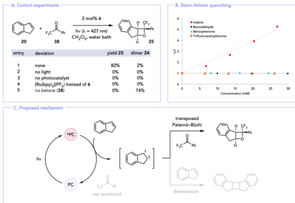
Fig. 5 Mechanistic studies for the transposed Paternò-Büchi reaction. (A) Control experiments. (B) Stern-Volmer quenching studies. (C) Proposed mechanism.
