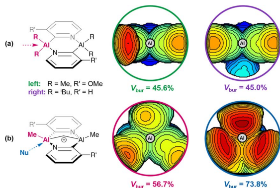
Fig. 12 Topographic steric maps showing the steric pressure exerted on each aluminium centre: (a) by the ring system in the neutral precatalysts 1c and 1d (left and right, respectively; viewed on the plane of the ring from the direction of the alkyl groups); (b) by the ring system in the active cationic catalyst 2a (viewed from the direction of the terminal methyl) (left) or by the entire ligand scaffold (including terminal alkyls, viewed from the direction of the incoming substrate) (right). The scale of the isocontours of altitude from the Al centre range between \pm 3.5 \text{ \AA} .
