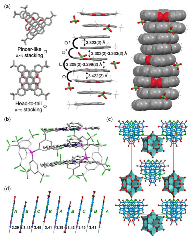
Fig. 20 (a) \pi - \pi stacking in the crystal structure of 60b_3(ClO_4)_2 \cdot THF \cdot (H_2O)_{0.5} ; (b) \pi -stacked trimer in the crystal structure of 61b_3^{2(\cdot+)}(BARF_4^-)_2 ; (c) a unit cell in the crystal structure of 62a_4^{3+}(PMo_{12}O_{40})^{3-} ; (d) \pi - \pi stacking in the crystal structure of 62a_4^{3+}(PMo_{12}O_{40})^{3-} . Reproduced with permission from ref. 110–112. Copyright 2020, 2023 and 2024 Wiley.
