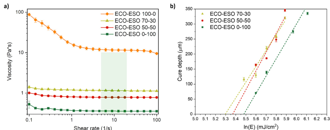
Fig. 6 Rheological behaviour with the green box representing the printability range for DLP/SLA 3D printing 12 (a) and working curves obtained with a 3D printer (b) of ECO-ESO formulations.
