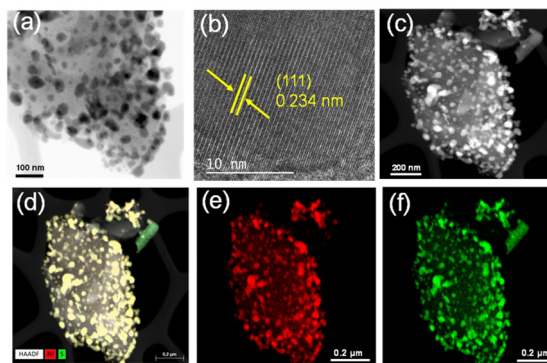
Fig. 2 (a) TEM overview image of Ni 3 S 2 /C (10 wt% Ni). (b) HRTEM image of a single nanoparticle, showing lattice fringes. (c) HAADF-STEM image with (d–f) EDXS of nanoparticles on the HAADF-STEM image in (c) with element maps of (d) combined Ni and S, (e) Ni (red) and (f) S (green).
