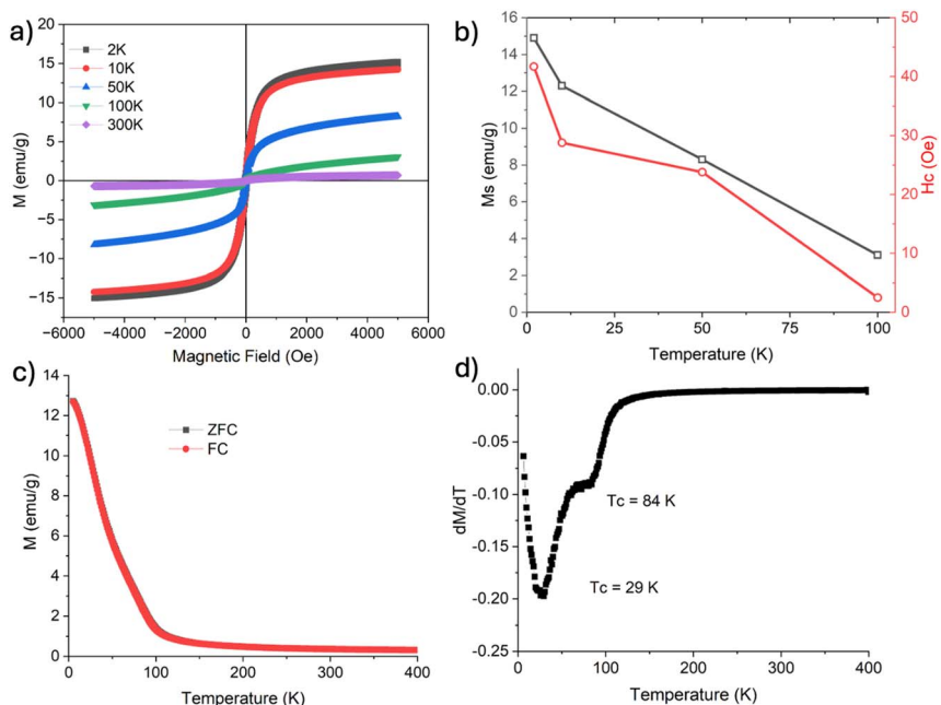
Fig. 8 Magnetic behaviour of the 90CRA condition. (a) M-H loops measured at 2, 10, 50, 100, and 300 K. (b) Temperature dependence of saturation magnetization ( M_s ) and coercivity ( H_c ), indicating a decrease in M_s and a decreasing trend in H_c with increasing temperature. (c) ZFC and FC magnetization curves recorded under a 1000 Oe field, showing a continuous decrease in magnetization with temperature. (d) dM/dT plot highlighting two magnetic transitions, with Curie temperatures identified at \sim 84 K and 29 K.
