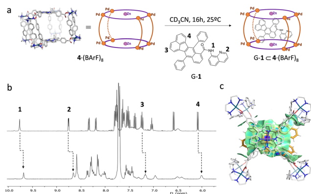
Fig. 1 (a) Schematic representation of the binding of G-1 within cage 4\cdot(\text{BArF})_8 . (b) Stacked partial ^1\text{H} NMR spectra of G-1 (top) and G-1\cdot 4\cdot(\text{BArF})_8 (bottom), showing spectral changes upon host-guest complexation. (c) Representation of non-covalent interaction (NCI) surface of encapsulated G-1 within the cage (weak van der Waals interactions in green and stronger interactions in blue).
