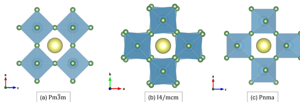
Fig. 1 Optimised structures of SrTiO 3 in the cubic Pm \bar{3} m (a), tetragonal I4/mcm (b) and orthorhombic Pnma phase (c). The I4/mcm and Pnma structures are oriented to show the equivalence to the cubic structure. 71 The Sr, Ti and O atoms are shown in yellow, light blue and green respectively. These images were prepared using the VESTA software. 72
