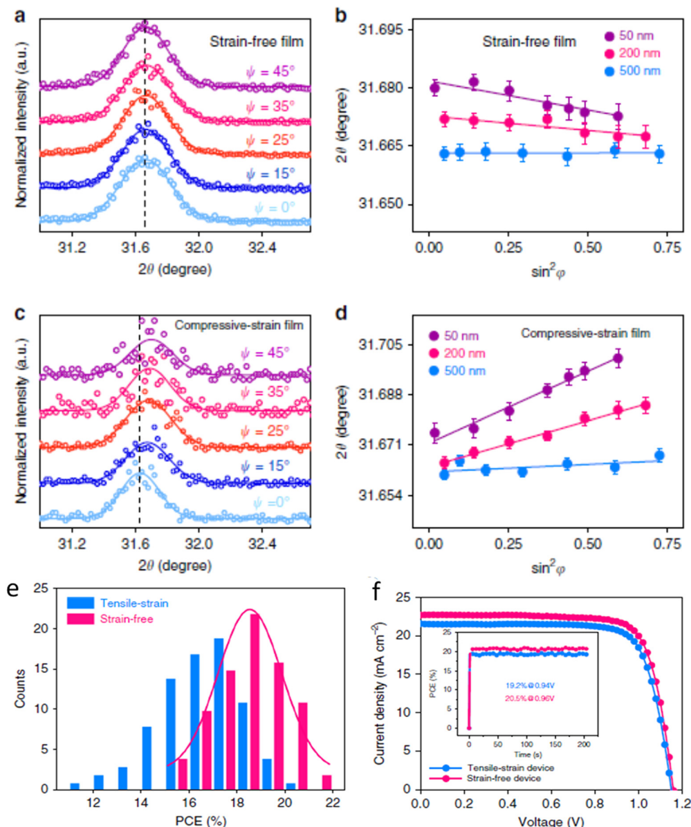
Fig. 12 The presence of Strain study in (FAPbI 3 ) 0.85 (MAPbBr 3 ) 0.15 . (a) Intensity vs. 2\theta for strain free sample, (b) 2\theta vs. \sin^2 function for strain free sample, (c) intensity vs. 2\theta for compressed strain, (d) 2\theta vs. \sin^2 function for compressed strain film, (e) Tensile strain vs. strain free, (f) current density vs. voltage for tensile strained and strain free film. Reproduced with permission. 333 Copyright 2019, Nature publishing group.
