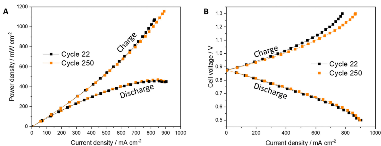
Fig. 5 Polarization measurements results of (A) power density and (B) cell's voltage of the RFB with SBGA at the beginning of life (Cycle 22) and after 250 cycles.
