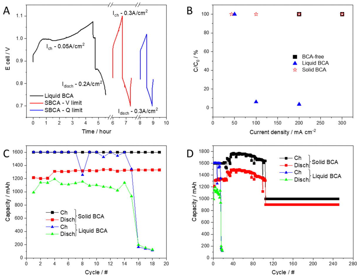
Fig. 4 (A) voltage profile of cell with liquid BCA and SBGA, (B) Ratio of the capacity C vs. initial capacity C_0 as a function of cycling current density for BCA-free, liquid and solid BCA, (C) and (D) Galvanostatic cycling with liquid BCA and SBGA.
