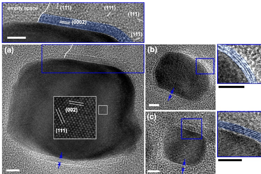
Fig. 4 HRTEM investigation of the NHD-700C,4h sample. The Fe–Ni NP in (a) sits at the edge of a hybrid cluster and is viewed along the [1\bar{M}x0\bar{O}31;0] zone axis. The \{111\} and \{002\} planes of the fcc FeNi alloy are indicated. In the magnified inset (a) top, the characteristic \{0002\} close-packed planes indicate the formation of few-layered graphite (blue pseudo colour) at the interface between the Fe–Ni NP and the carbon nanotemplate. Close-packed \{111\} planes, coming from small ND crystallites, are also indicated. The white line delineates the border of the ND nanotemplate. HRTEM images of other Fe–Ni metallic NPs, showing the formation of few-layered graphite of similar thickness (b) and (c). All scale bars correspond to 5 nm.
