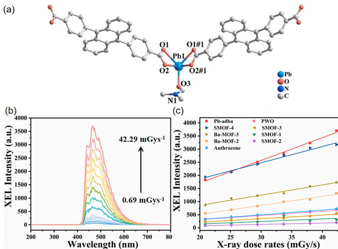
Fig. 11 (a) Coordination environments of the \text{Pb}^{2+} ion. (b) The XEL spectra in the dose rate range of 0.69\text{--}42.29 \text{ mGys}^{-1} at a voltage of 50 kV. (c) Linear correlation between XEL intensity and dose rate for Pb-adba , PWO, anthracene crystals, and other documented scintillating MOFs. Reprinted with permission. 60 Copyright 2022 Elsevier.
