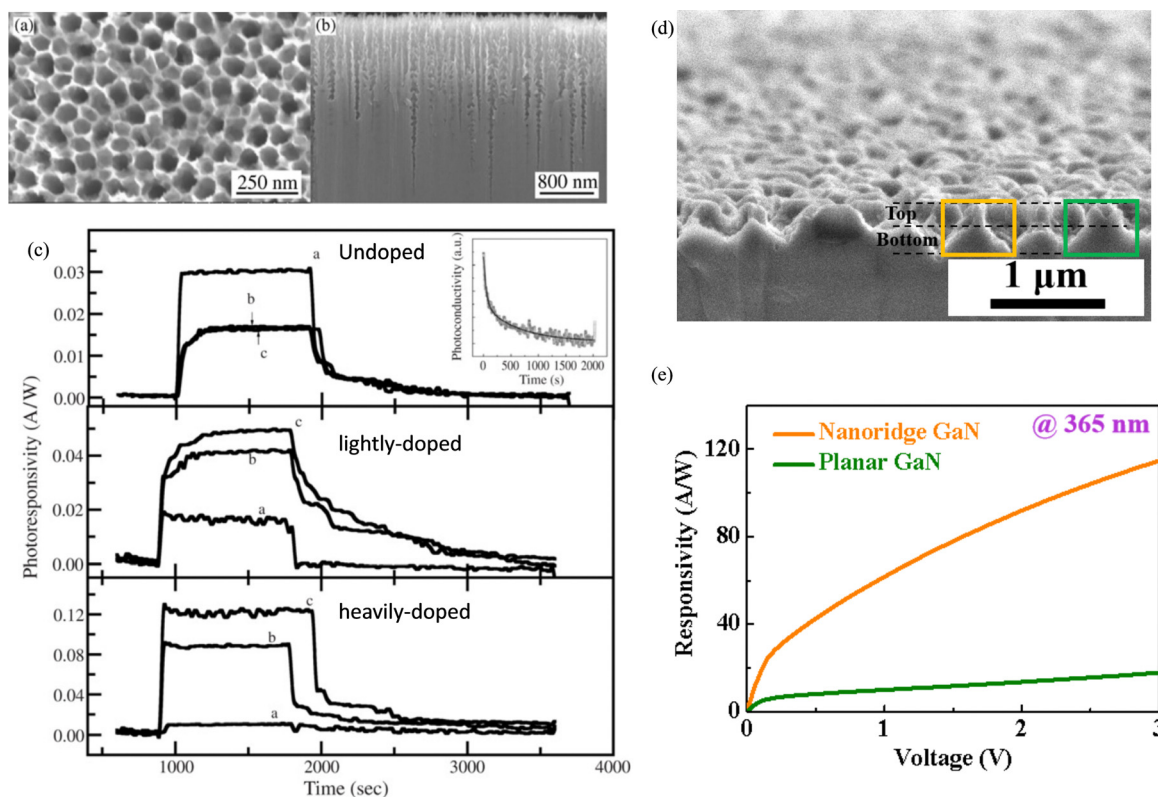
Fig. 22 (a) Top and (b) cross-sectional SEM images of GaN porous structures. (c) Photoresponse of MSM PDs based on GaN samples with different doping concentrations indicated in subfigures. Curves labeled as (a), (b) and (c) correspond to unetched, 1-hour etched, and 2-hour etched GaN samples, respectively. Reproduced with permission. 139 Copyright 2006, Elsevier. (d) Cross-sectional SEM images of GaN nanoridge structures. (e) UV photoresponse of MSM PDs based on planar and nanoridge textured GaN surfaces. Reproduced with permission. 128 Copyright 2023, American Chemical Society.
