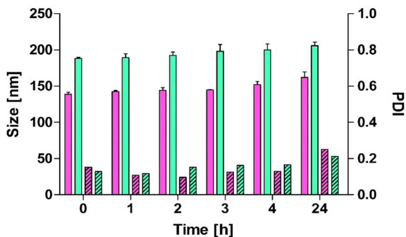
Fig. 2 Size (filled bars) and PDI (striped) of liposomes (pink) and pp-liposomes (green) in 25 mM HEPES buffer at indicated time points at 37 °C. Data are shown as mean \pm SD ( n = 3 ).
