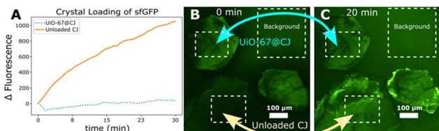
Fig. 5 (A) Change in fluorescence over time for 2 crystals and the background. 2 crystals are monitored for their change in fluorescence (accumulation of sGFP, ROI highlighted with white dotted boxes) over time. (B) A confocal image of the crystals (both UiO-67 loaded and not) as soon as the sGFP is added. ROI's are shown in white dotted boxes for each region, corresponding to the labels in panel (A). (C) The same crystals 20 minutes later, allowing sufficient time for sGFP to diffuse into the pores of the CJ crystals.
