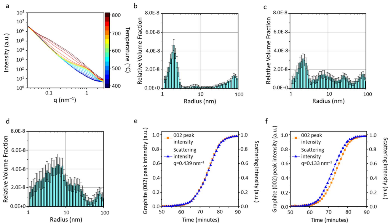
Fig. 5 (a) SAXS data for the heating range 400–800 ^\circ\text{C} and corresponding particle size histograms for data scans at (b) 700 ^\circ\text{C} , (c) 750 ^\circ\text{C} and (d) 800 ^\circ\text{C} for cellulose- \text{Fe}(\text{NO}_3)_3 . Normalised graphite (002) peak intensity alongside scattering intensity at (e) q = 0.439 \text{ nm}^{-1} and (f) q = 0.133 \text{ nm}^{-1} .
