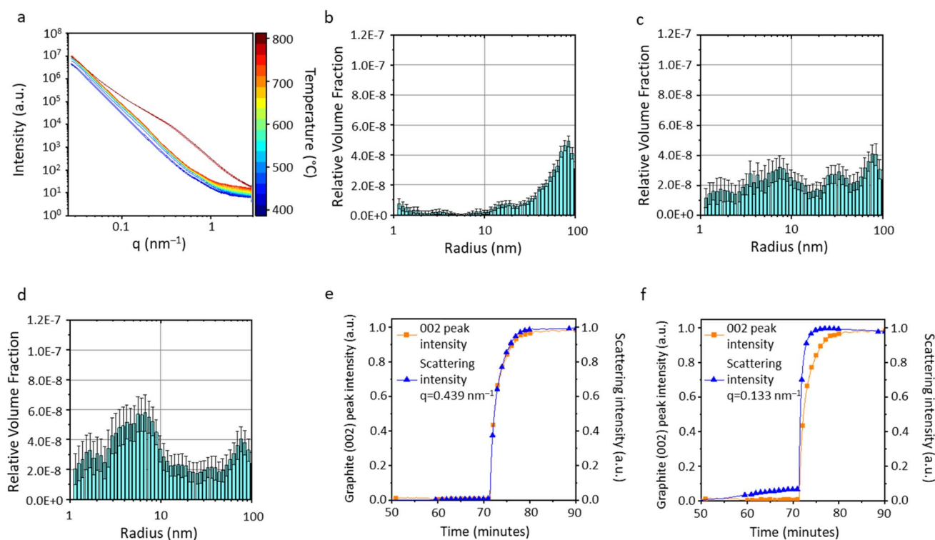
Fig. 6 (a) SAXS data for the heating range 400–800 ^\circ\text{C} and corresponding particle size histograms for data at (b) 750 ^\circ\text{C} , (c) 760 ^\circ\text{C} and (d) 770 ^\circ\text{C} for cellulose- \text{FeCl}_3 . Normalised graphite (002) peak intensity alongside scattering intensity at (e) q = 0.439 \text{ nm}^{-1} and (f) q = 0.133 \text{ nm}^{-1} .
