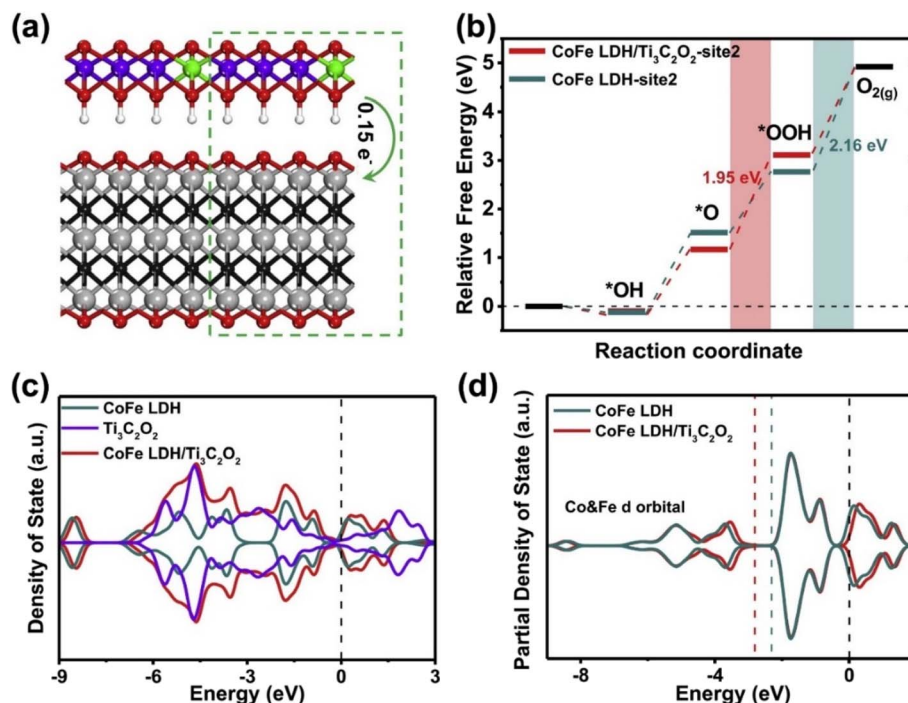
Fig. 28 (a) Side view of optimized CoFe LDH/Ti 3 C 2 O 2 (2 × 1 × 1 cell) with color-coded elements. (b) Free energy diagrams for OER at 0 V on CoFe LDH and CoFe LDH/Ti 3 C 2 O 2 . (c) DOS of CoFe LDH/Ti 3 C 2 O 2 , CoFe LDH, and Ti 3 C 2 O 2 , with Fermi level at zero. (d) PDOS of 3d orbitals for Co and Fe in CoFe LDH and CoFe LDH/Ti 3 C 2 O 2 , showing d-band centers. Reproduced from ref. 126 with permission from Elsevier Ltd, copyright © 2021.
