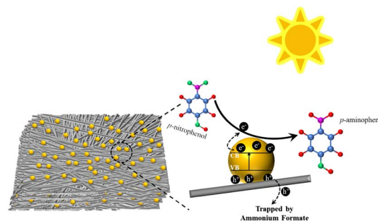
Fig. 8 Possible mechanism of photocatalytic reduction of p -NP under simulated solar light. Reprinted with permission from ref. 95. Copyright 2021, Royal Society of Chemistry.
