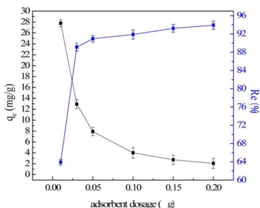
Fig. 13 Effect of adsorbent dosage ( V = 50 mL; T = 25 \pm 1 °C; C_0 = 10 mg L; q_e is the equilibrium adsorption capacity). 64 Copyright 2016, John Wiley and Sons.
