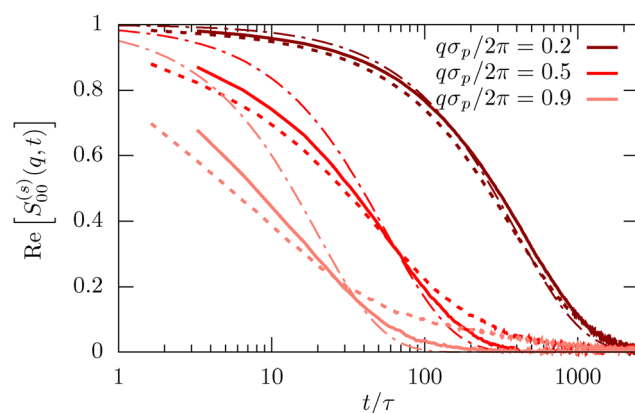
Fig. 5 Incoherent scattering function S_{00}^{(s)}(q, t) for the lowest mode \mu = \nu = 0 for \phi = 0.32 and L = 1.9\sigma_p . Results for different wave numbers q are obtained from confocal microscopy experiments (full lines), MD simulations (dotted lines) and the diffusive approximation eqn (13) using the diffusion coefficient D extracted from experiments, as shown in Fig. 2.
