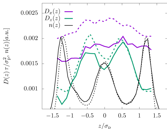
Fig. 3 Position-dependent diffusion coefficient D(z) , as defined in eqn (5) and (6) for the dense system ( \phi = 0.32 ) and L = 2.4\sigma_p . Shown are the in-plane coefficient, D_x(z) , the lateral coefficient, D_z(z) , as well as the density profile n(z) .
