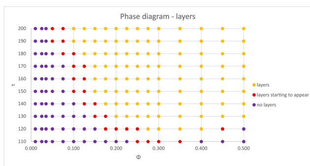
Fig. 7 Phase diagram in the (\phi, \tau) plane, detailing the layering formation along the transversal direction, obtained via MD simulations. The interactions are fully screened, and the monopole charge is set at Z = 90 .
