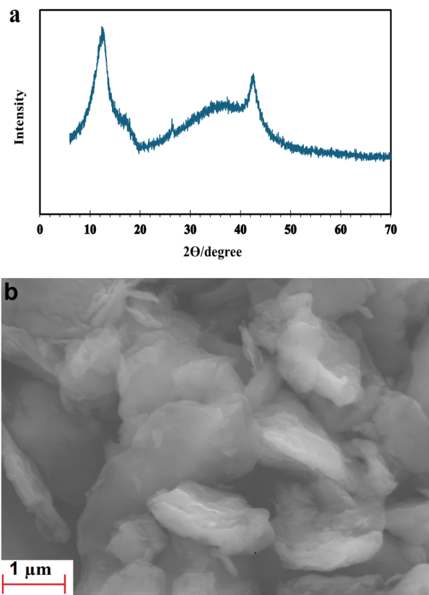
Fig. 2 (a) XRD pattern and (b) SEM image of graphene oxide.
