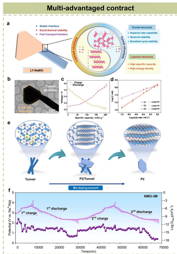
Fig. 8 (a) A schematic diagram, (b) TEM image, (c) GITT plots, and (d) \log(i) vs. \log(v) plots for Na 0.6 MnO 2 . 110 Copyright 2023, American Chemical Society. (e) A schematic diagram of the phase transition process for Na 0.44 Mn 1-x Mo x O 2 with increasing Mo content. (f) GITT curves and corresponding Na ion diffusion coefficients for NMO-3M. 111 Copyright 2024, Elsevier.
