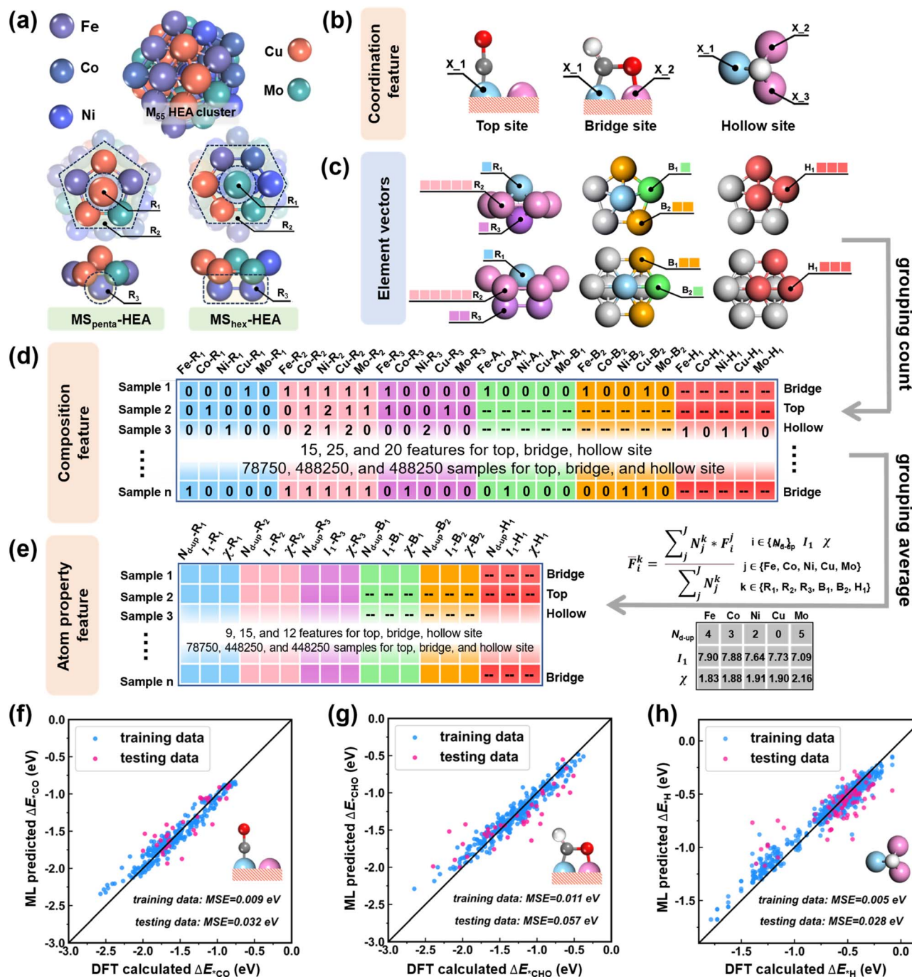
Fig. 1 (a) Structure of FeCoNiCuMo HEA clusters, with top and side views of microstructures ( MS_{penta} -HEAs and MS_{hex} -HEAs). The different regions of the microstructures ( R_1 , R_2 , and R_3 ) have been outlined. (b) Coordination features extracted from top (*CO), bridge (*CHO), and hollow (*H) sites. (c) Element vectors extracted from 6 regions ( R_1 , R_2 , R_3 , B_1 , B_2 , and H_1 ) on MS_{penta} -HEAs and MS_{hex} -HEAs. (d) Composition features converted from element vectors by group counting of different elements in different regions. (e) Atomic property features generated from the composition features by grouping the average for atomic properties in different regions. Plots of DFT-calculated vs. ML-predicted values of (f) \Delta E_{CO} , (g) \Delta E_{CHO} , and (h) \Delta E_H , and the mean square errors (MSEs) of training and testing sets for model evaluation.
