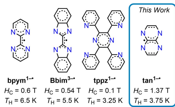
Fig. 1 Selected radical ligands used to construct dinuclear dysprosium single-molecule magnets [(\text{Cp}^*_2\text{Dy})_2(\mu\text{-L})]\text{X} with coercive fields ( H_C ) and open magnetic hysteresis loops at or below this temperature ( T_H ) under conventional sweep rates. Ligands L are: \text{bpym} = 2,2'-bi-pyrimidine ( \text{X} = \text{BPh}_4^- ), \text{Bbim} = 2,2'-bisbenzimidazole ( \text{X} = [\text{K}(\text{crypt-222})]^+ , \text{crypt-222} = 2.2.2-cryptand), \text{tppz} = 2,3,5,6-tetra(2-pyridyl)pyrazine ( \text{X} = \text{BPh}_4^- ), \text{tan} = 1,4,5,8-tetraazanaphthalene ( \text{X} = \text{BARf}_{20}^- ).
