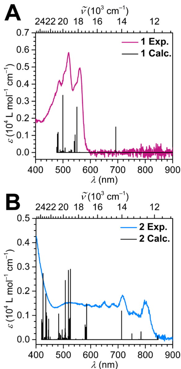
Fig. 5 UV-vis spectra of (A) [(\text{Cp}^*\text{2Dy})_2(\mu\text{-tan})] (1) (pink line), and of (B) [(\text{Cp}^*\text{2Dy})_2(\mu\text{-tan})][\text{BARF}_{20}] (2) (blue line), recorded at 32 \mu\text{mol L}^{-1} (1) and 140 \mu\text{mol L}^{-1} (2) concentrations in DCM at room temperature. Black vertical lines represent calculated TD-DFT transitions.
